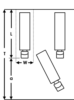
90-Degree Docks
