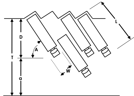
Sawtooth Docks
