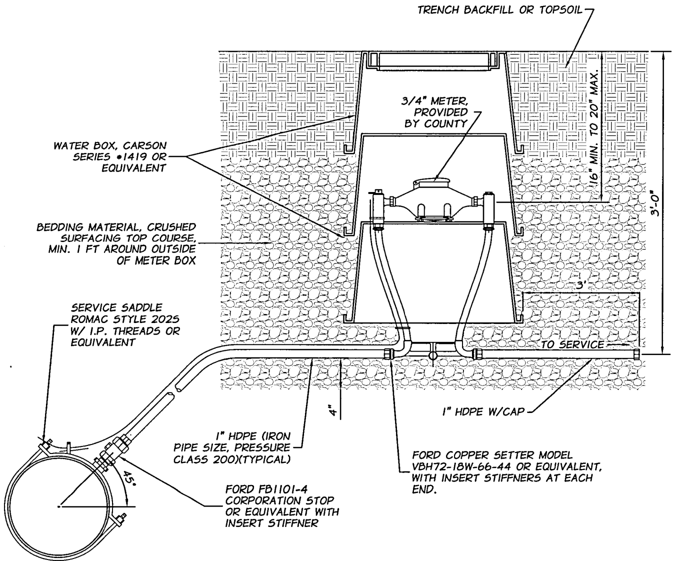
CROSS SECTION NTS
