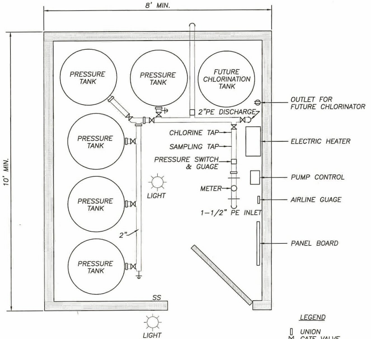
PIPING SCHEMATIC NTS
