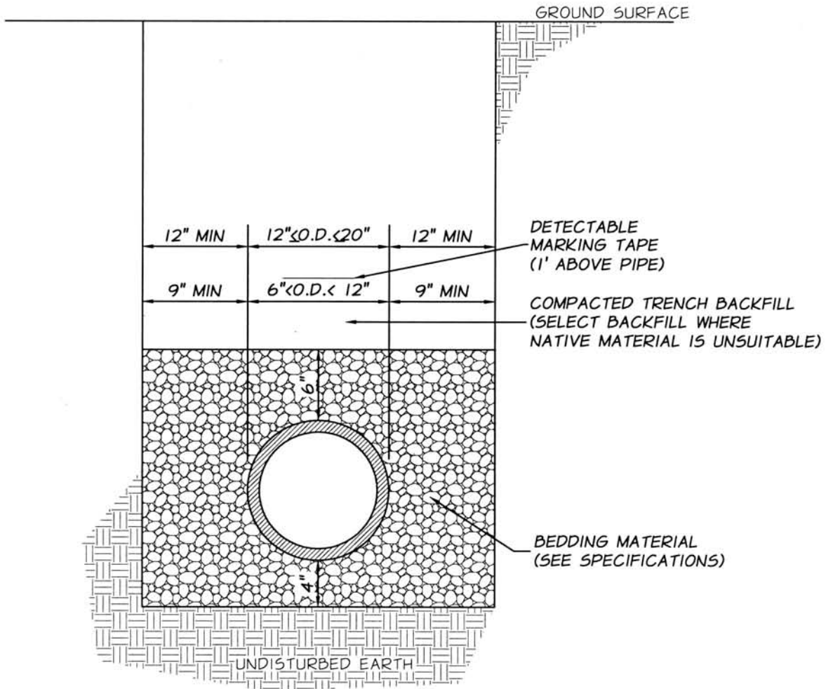
CROSS SECTION NTS
