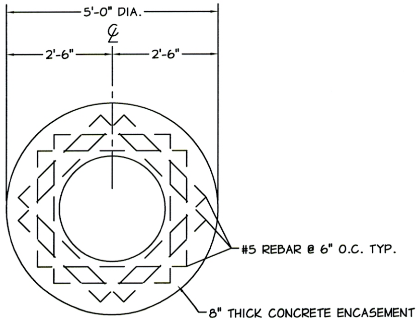
PLAN OF CONCRETE ENCASEMENT
