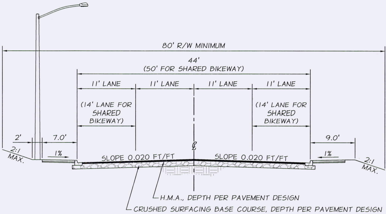
CROSS SECTION NTS
