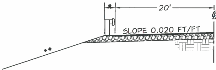
CROSS SECTION NTS
