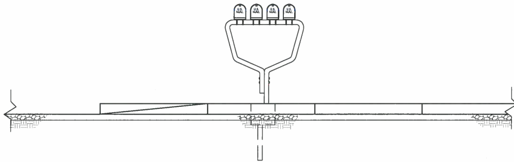
ELEVATION VIEW NTS MAILBOX WIDENING DETAIL
