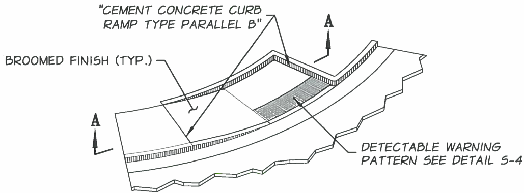
PARALLEL CURB RAMP DETAIL NTS
