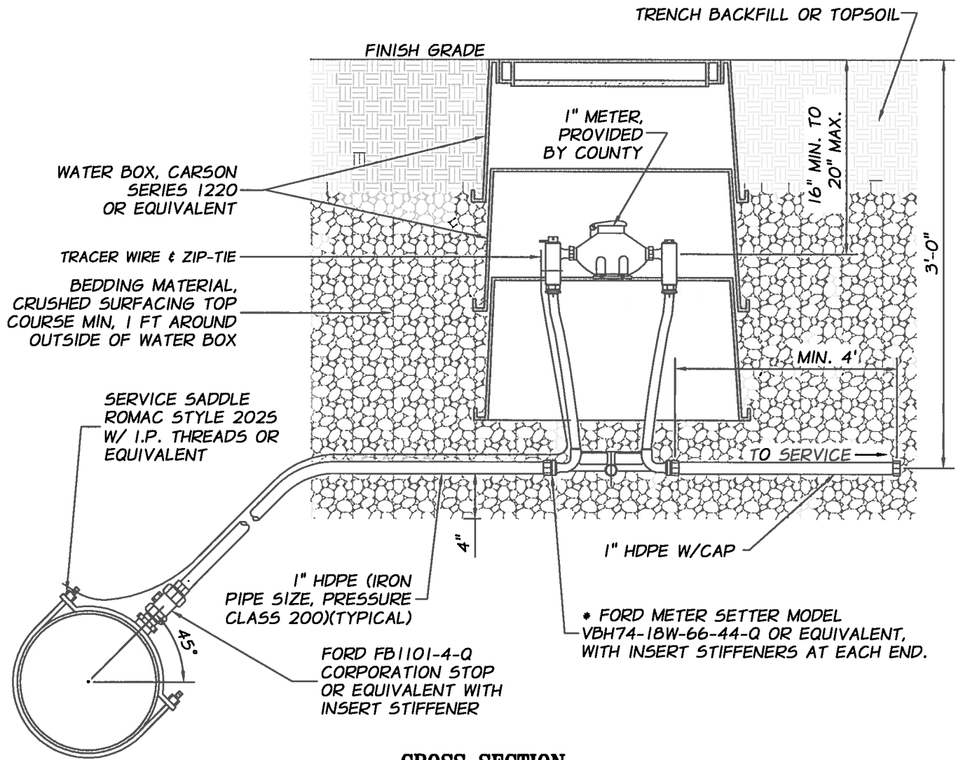
CROSS SECTION NTS
